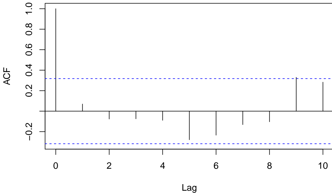
ACF for Q2 residuals
