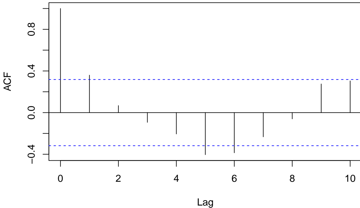
ACF for Q4 residuals
