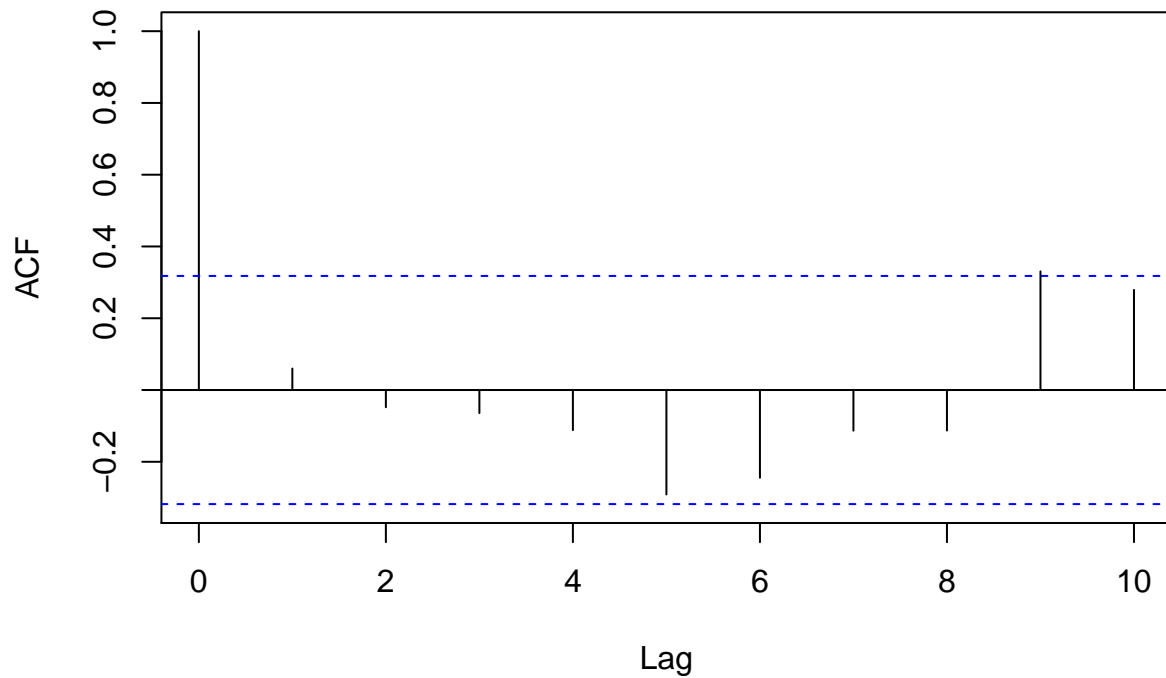
ACF for Q1 residuals
