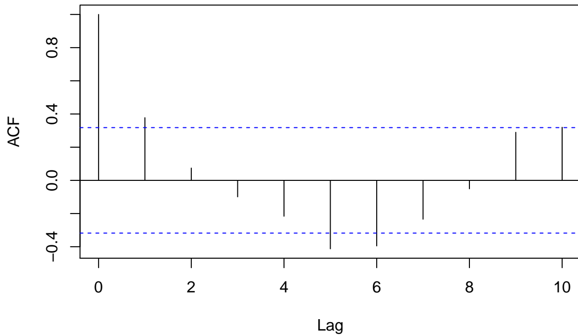
ACF for Q3 residuals
